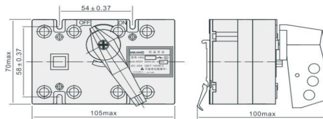
BRHGL-63/3(4) 隔离开关的外形尺寸及安装尺寸
